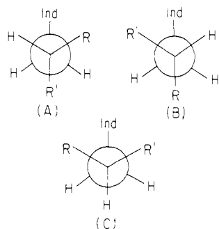
Figure 2. A, B, and C conformers about the C ^{\alpha} -C ^{\beta} tryptophyl bond: Trp, R = NH _3^+ , R' = CO _2^- ; EE, R = COOEt, R' = COOEt; NATE, R = NHCOCH _3 , R' = COOEt; AE, R = CONH _2 , R' = COOEt; NATA, R = NHCOCH _3 , R' = CONH _2 ; AA, R = CONH _2 , R' = CONH _2 .
